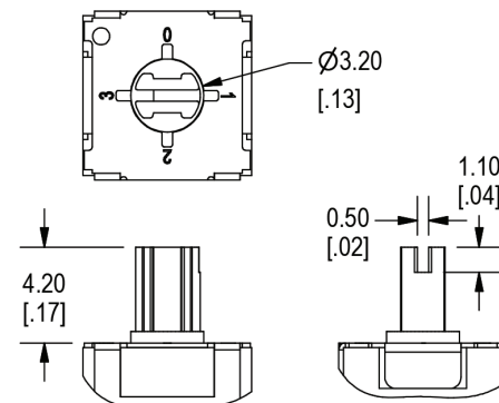
C - Slot, Flat 4.2mm
