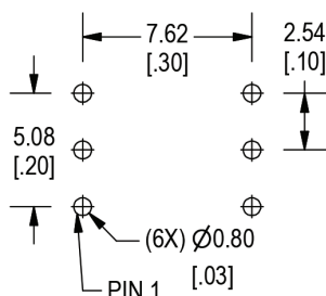
T - Through Hole PC Pin
