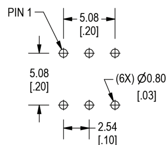
VB - Right Angle PC Pin, 5.08mm spacing
