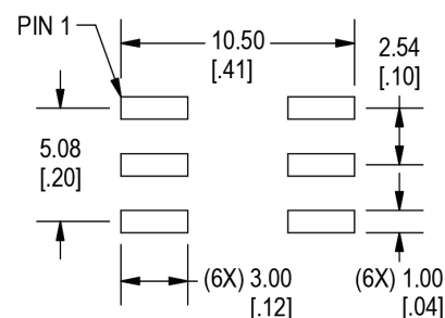
G - Gull Wing, Surface Mount
